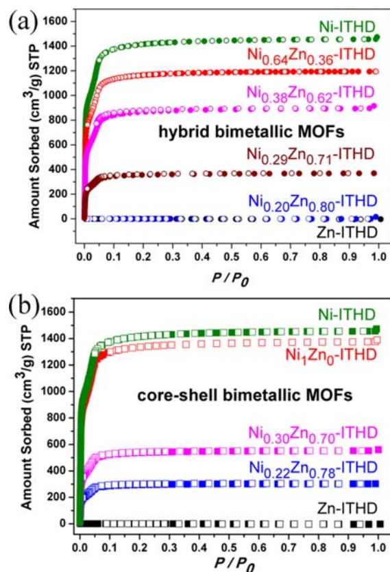
Figure 6. The N_2 sorption isotherms of (a) hybrid bimetallic Ni_xZn_{1-x} -ITHDs (circles) and (b) core-shell bimetallic Ni_xZn_{1-x} -ITHDs 11 (squares) at 77 K. Solid and open shapes represent adsorption and desorption isotherms, respectively.
