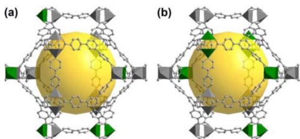
Figure 5. Two proposed hybrid bimetallic Ni_xM_{1-x} -ITHD structures, where M = Zn(II) and Co(II) . (a) The framework with both homodinuclear paddle-wheel SBUs M_2(COO)_4 and Ni_2(COO)_4 and heterodinuclear SBU NiM(COO)_4 . (b) The framework with only the homodinuclear SBUs. Ni polyhedra (green), Zn, and Co polyhedra (gray).
